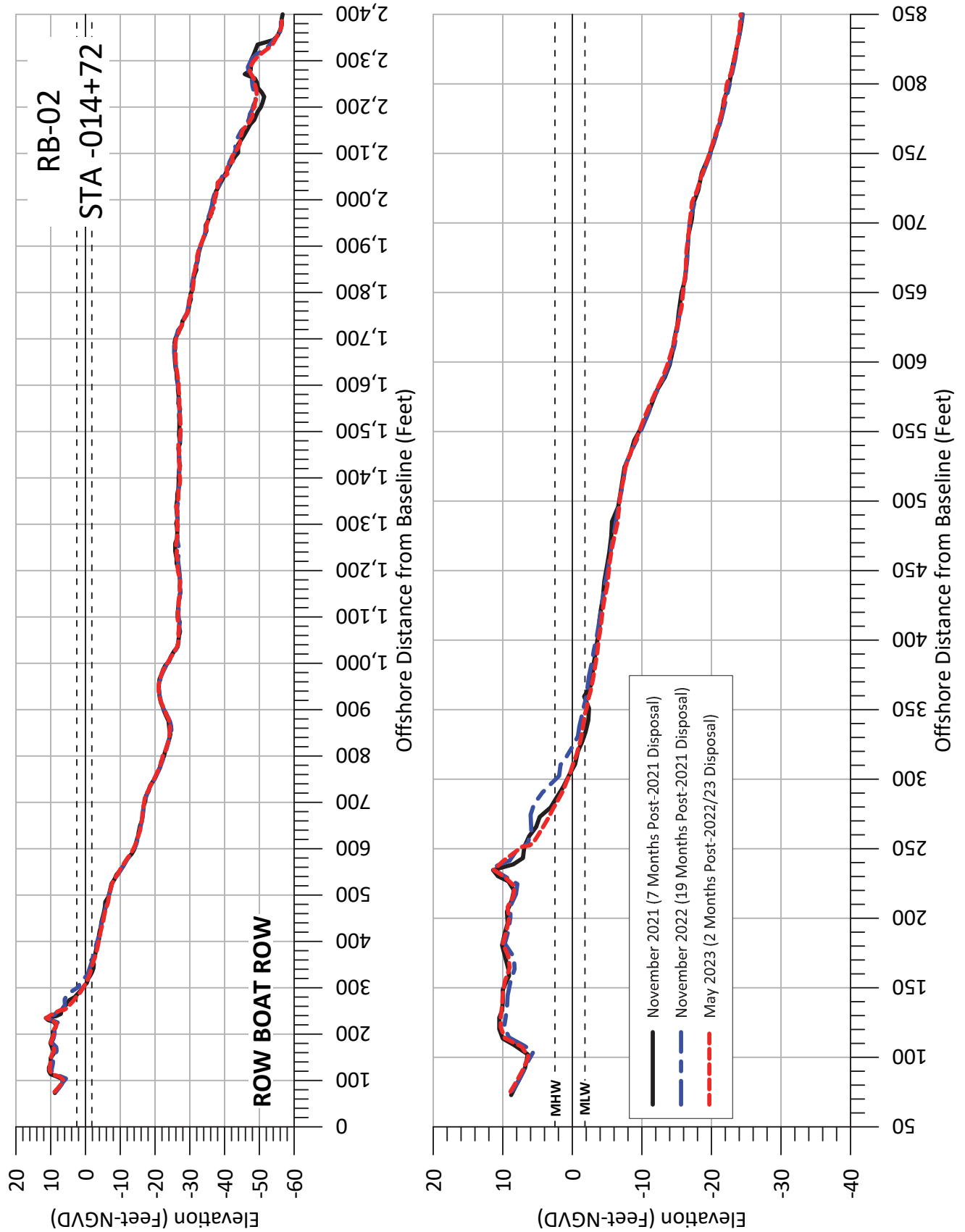
Figure A-02: Measured beach profiles at baseline Station -014+72 , Bald Head Island, N.C.
