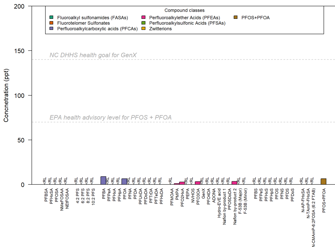
Figure 1: Concentrations of individual PFAS compounds.
