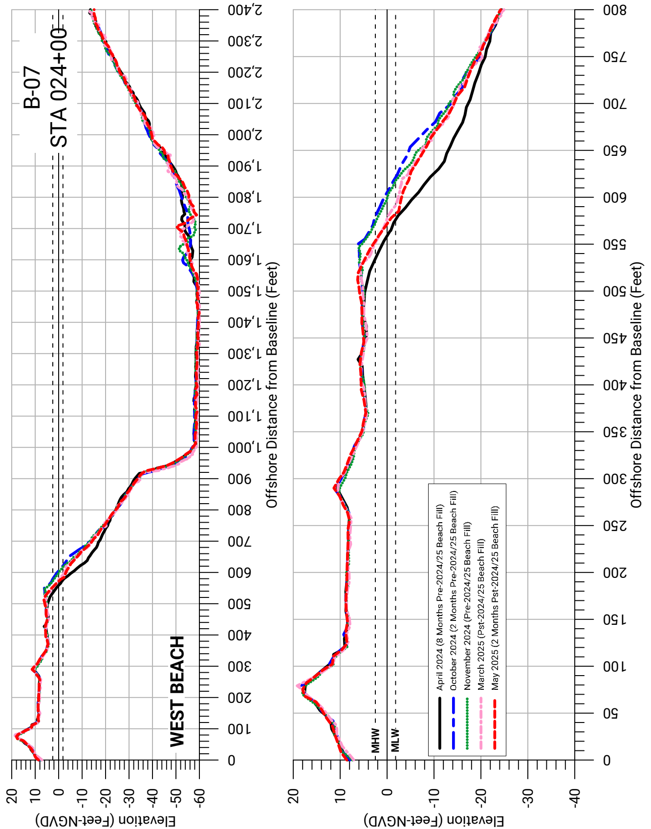
Figure G-15: Measured beach profiles at baseline Station 024+00 , Bald Head Island, N.C.
