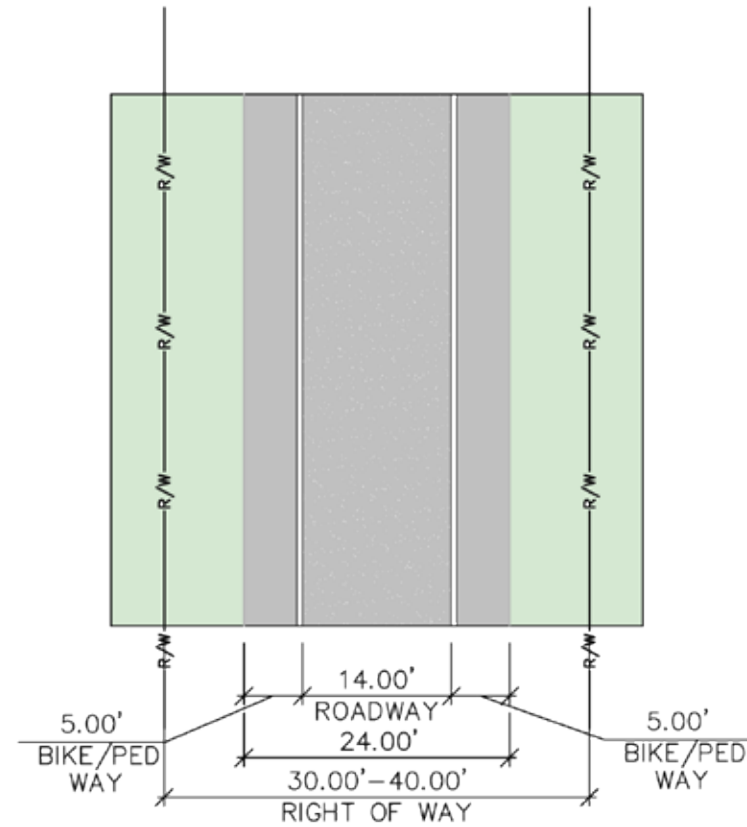
PROPOSED PLAN
