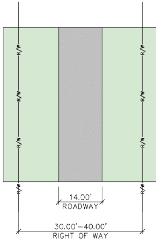
EXISTING PLAN
